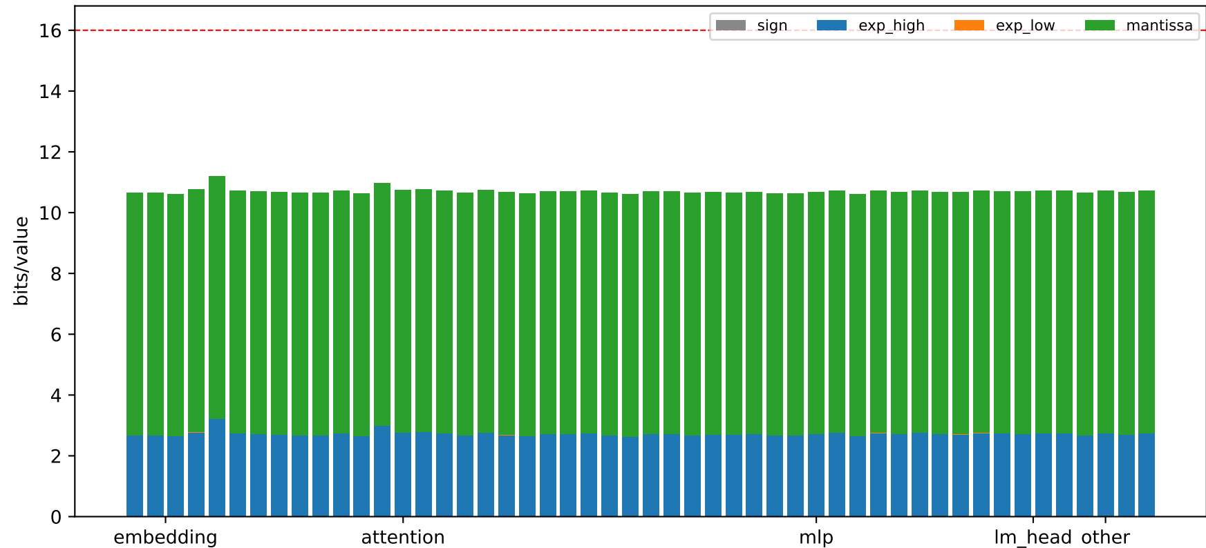
Fig 1 — bf16 byte-marginal entropy decomposition by tensor category
