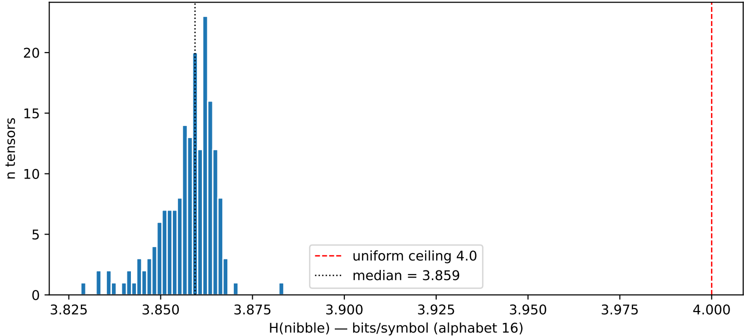
Q4_K nibble entropy — precheck atlas (n = 180 tensors from training-source Qwen2.5-0.5B GGUF)
